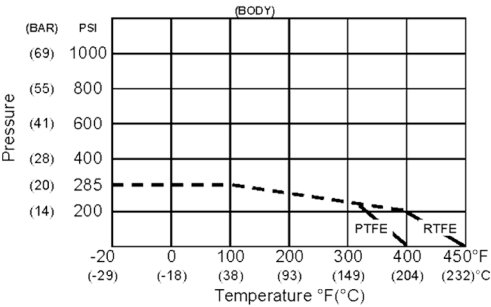
PRESSURE TEMPERATURE RATINGS
